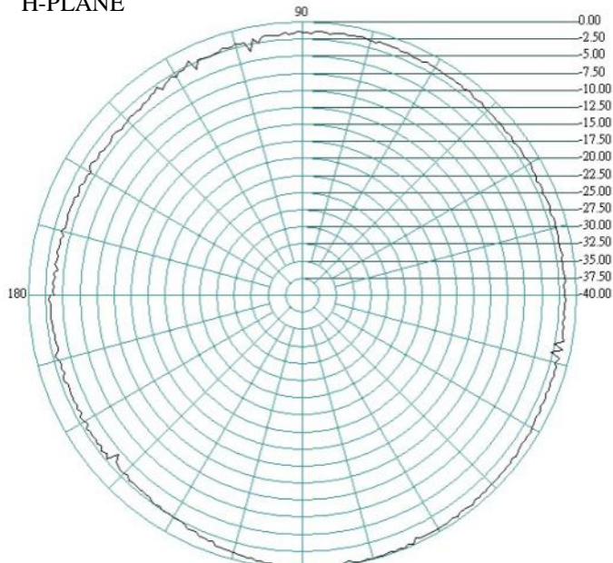
Antenna Pattern
