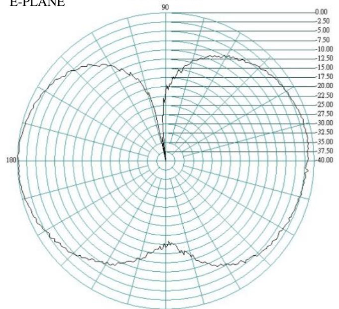
Antenna Pattern
